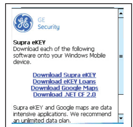
Windows screenshot
